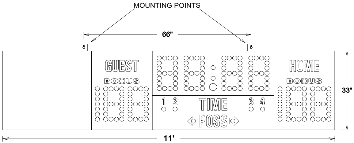
Figure 2 MP-269 Mounting Points
