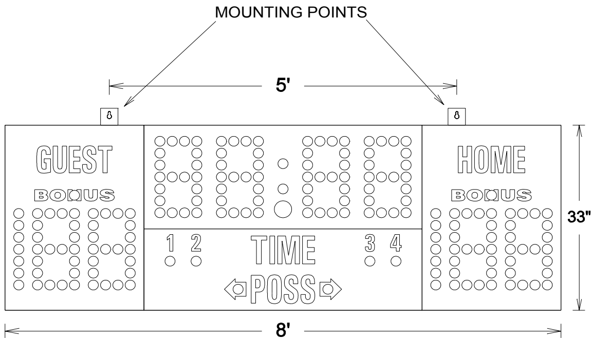
Figure 1 MP-259 Mounting Points
